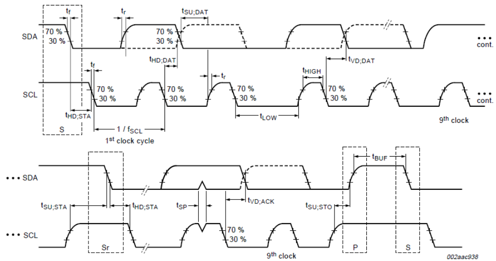
Figure 1 I2C TIMING DIAGRAM
