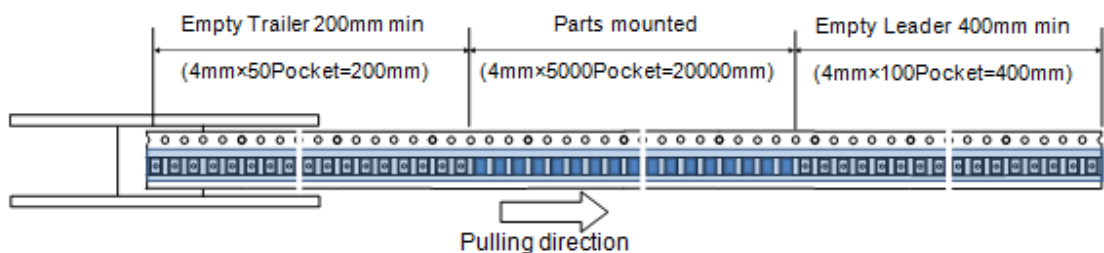
Figure 14 Pulling direction and Trailer/Leader
