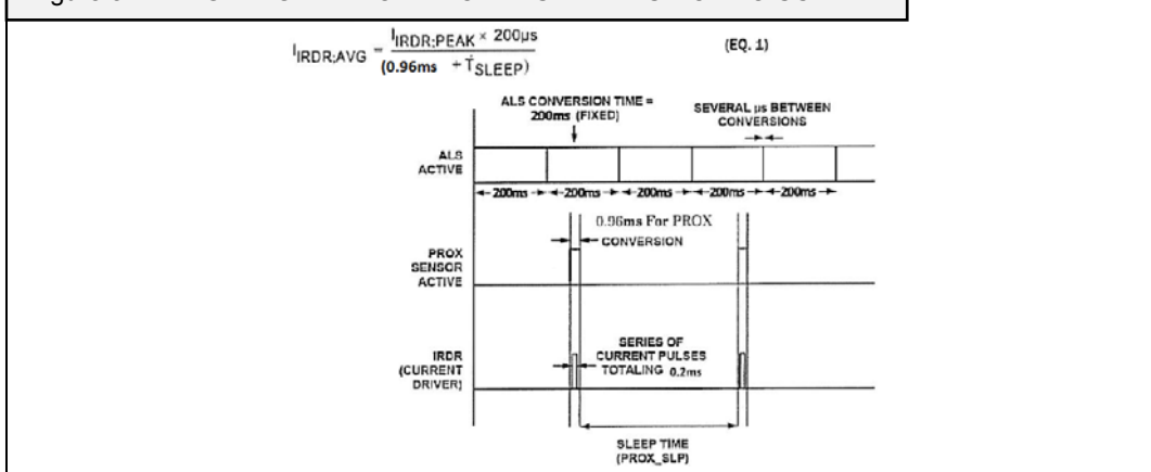
Figure 8 TIMING DIAGRAM FOR PROX/ALS EVENTS NOT TO SCALE
