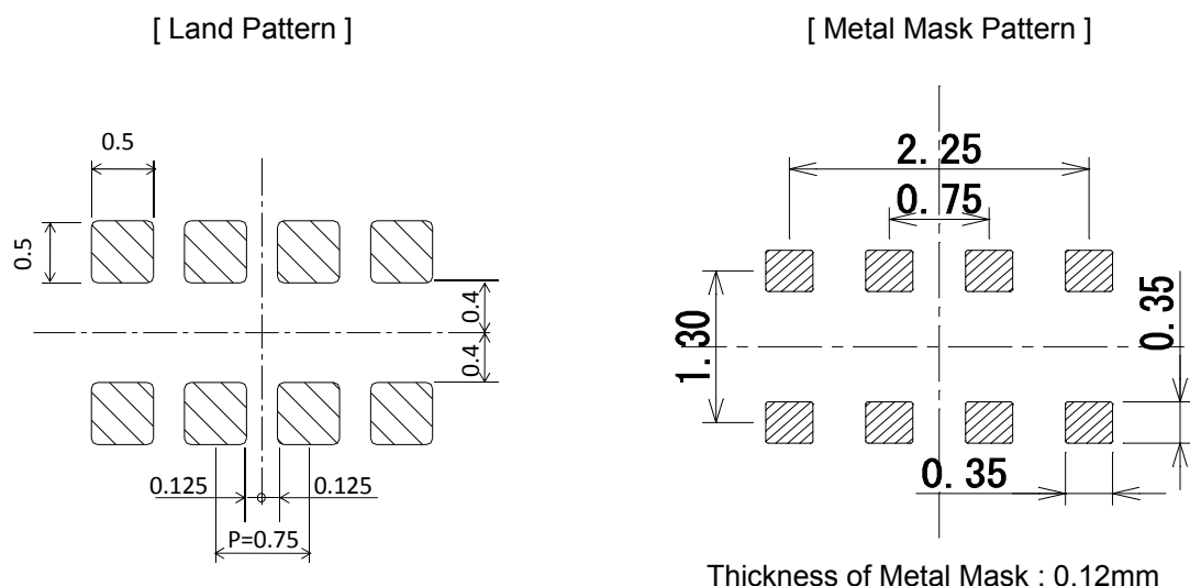
Figure 11 Recommended Land and Metal Mask pattern
