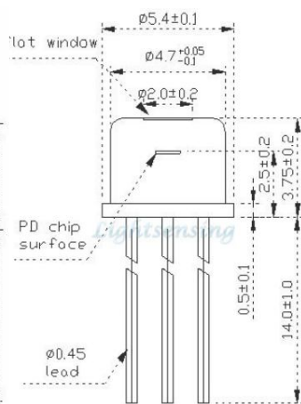
2mm Flat window 3PIN TO Model: 0
