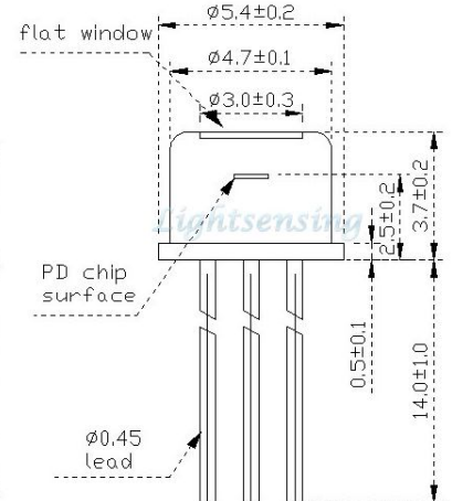
3mm Flat window 3PIN TO Model: 03
