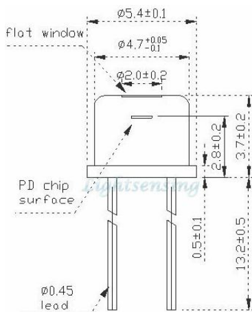
2mm Flat window 2PIN TO Model: 0
