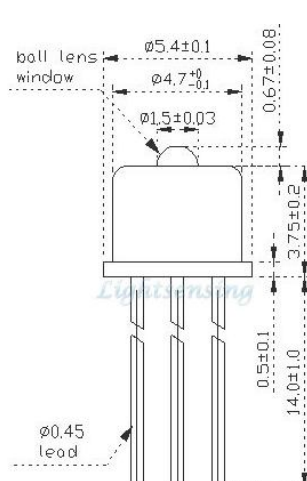
Standard ball lens cap 3PIN TO Model: 1
