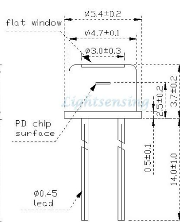
3mm Flat window 2PIN TO Model: 03
