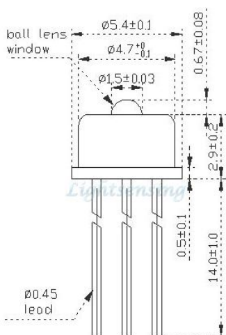
Short ball lens cap 3PIN TO Model: S1
